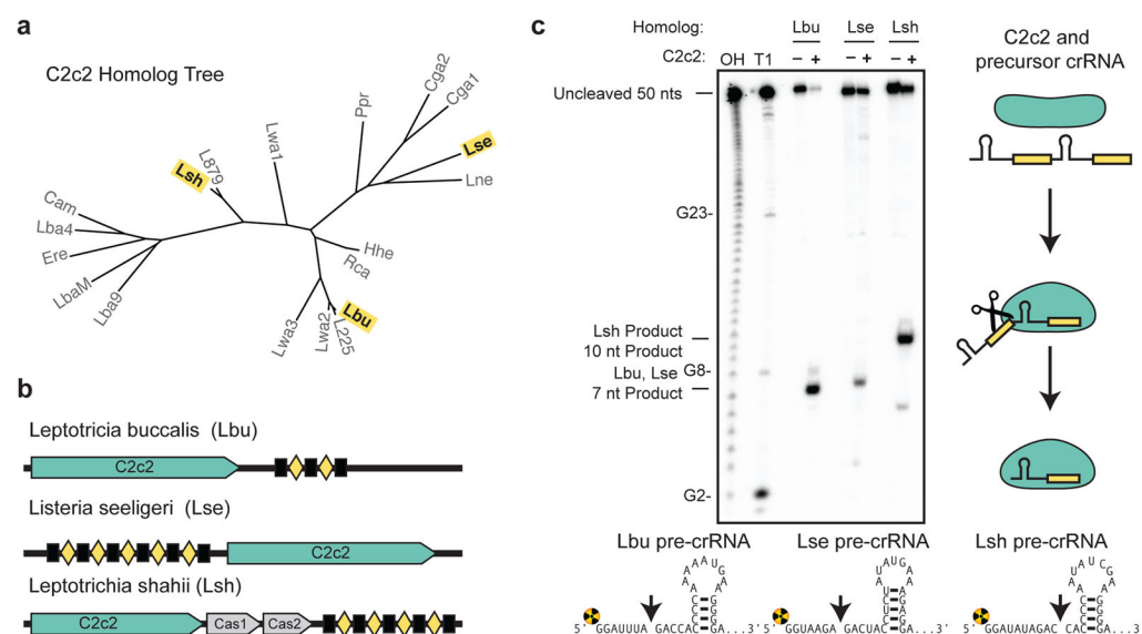
Figure 1. C2c2 proteins process precursor crRNA transcripts to generate mature crRNAs
